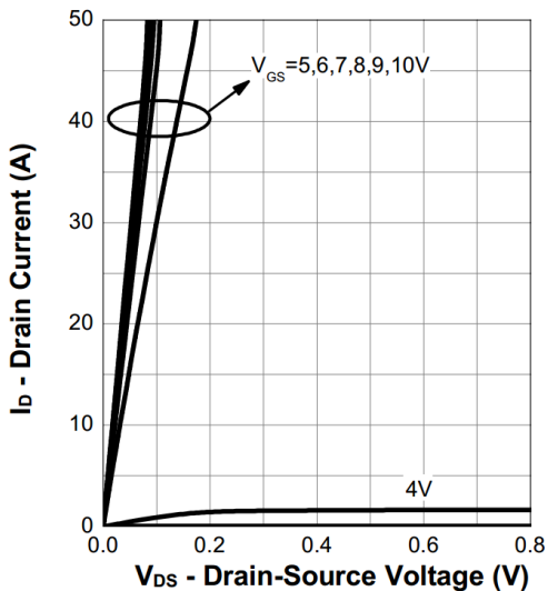
5. Output Characteristics
