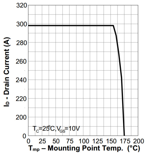
2. Current Capability
