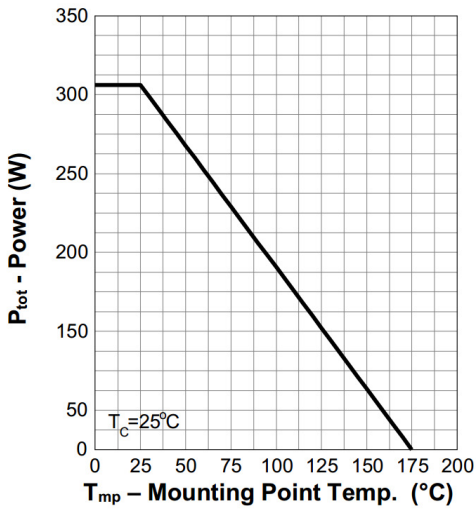
1. Power Capability
