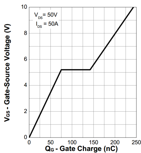
12. Gate Charge
