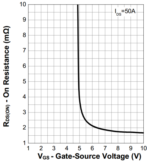
7. Transfer Characteristics
