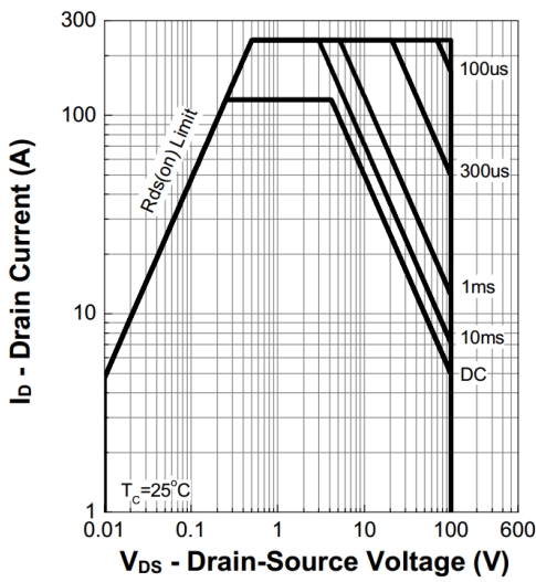
3. Safe Operating Area
